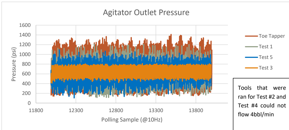
Figure 1 Pressure pulse profiles for tools tested
