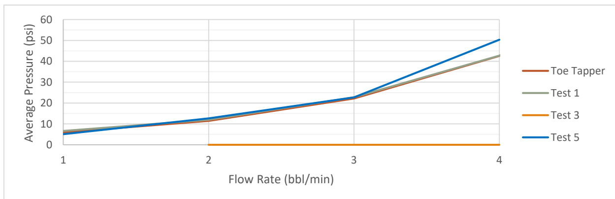
Figure 2 Average Pressure drops across tested tools
